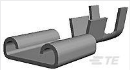
TE 产品编号160808-2 250 FASTON,REC.,17-14 AWG,BR
