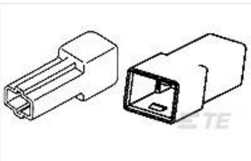
TE 产品编号880309-1 1 WAY FF 250 HOUSING TAB NYLON 6.6 NAT
