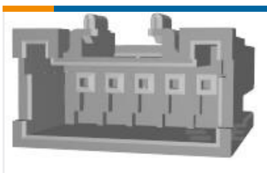
TE 产品编号316089-1 2.5 SIGNAL DBL LOCK CAP HSG 5P
