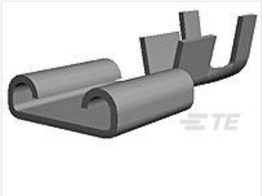
TE 产品编号170180-2 205 FASTON,REC.,18-14 AWG,TPBR
