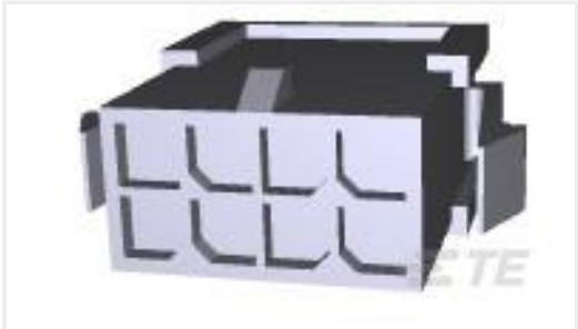
TE 产品编号794615-8 PANEL MT DBL ROW HSG 8 POS
