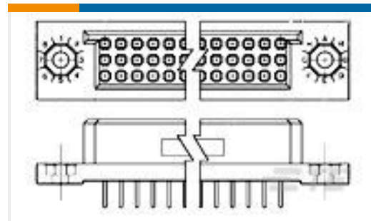
TE 产品编号533287-3 BOX II 3 ROW RECP ASSY 96 POS
