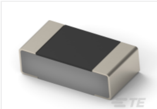
TE 产品编号3-2176467-0 TLRP 1206 1.0W R020 1% 100PPM 5K RL
