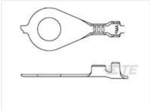
TE 产品编号880661-3 RING TONGUE 0.5-1.0 MM2 0.61X14.60 TPBR
