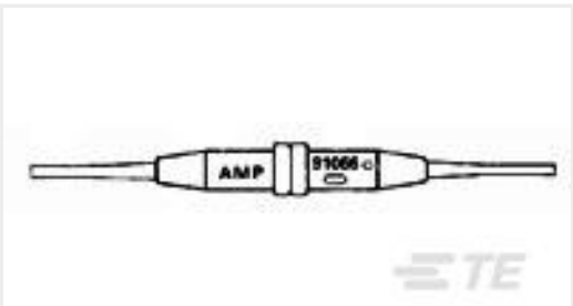
TE 产品编号91066-3 INSERTION/EXTRACTION TOOL
