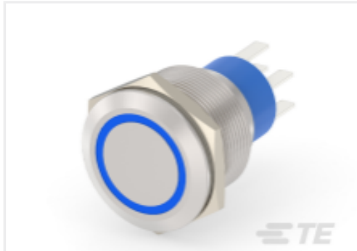
TE 产品编号7-2213772-9 AV22 DPL 3A MOVE RING LED BLUE 24V
