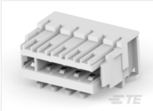
TE 产品编号2-2306286-5 5P DUOPLUG MARK II SIDE LOCKING, FUL
