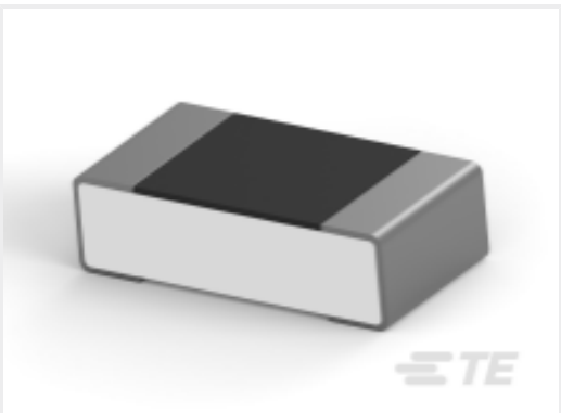
TE 产品编号2-2176365-5 RQ 0603 71R5 0.1% 10PPM 1K RL
