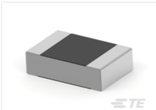
TE 产品编号5-2176238-6 CPF A 0805 25K 0.1% 25PPM 5K RL
