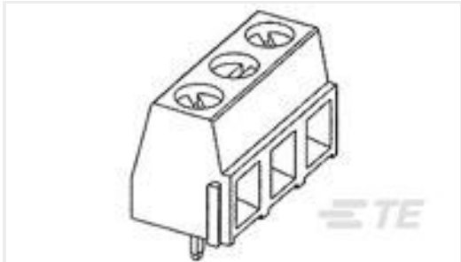
TE 产品编号282837-8 TERMI-BLOK PCB MOUNT 8P
