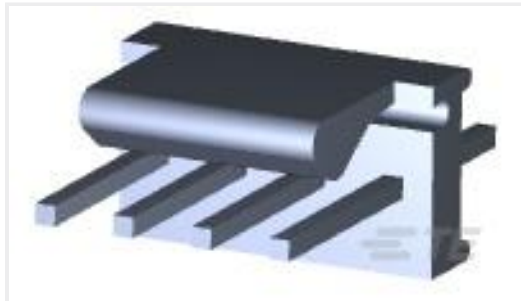
TE 产品编号3-641126-4 04P MTA100 HDR ASY FL/STR LF
