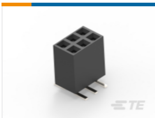
TE 产品编号2271646-6 AMPMODU, REC, 2.54, DR, SMT, 9.90 H, 6POS
