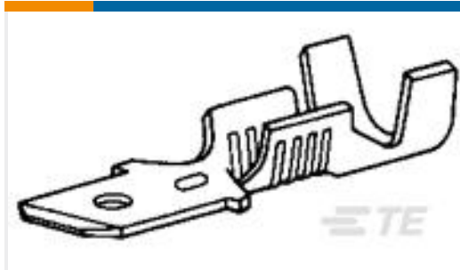
TE 产品编号62531-1 205 FASTON TAB 18-14 AWG TPBR
