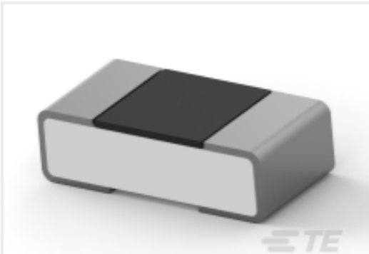
TE 产品编号2-2176364-3 RQ 0402 7K87 0.1% 10PPM 5K RL
