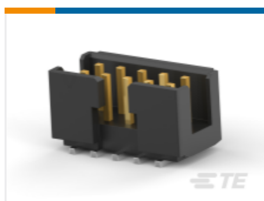
TE 产品编号1-2373376-0 10P,2MM,SHRD HDR,DRV,T,SMD,0.1 AU,TB
