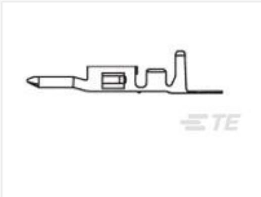
TE 产品编号794955-1 VAL-U-LOK PIN BR SN 22-18AWG NAT
