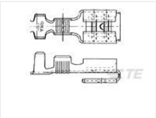
TE 产品编号160739-1 250 FASTON,PIGGYBACK REC.,18-14 AWG,BR
