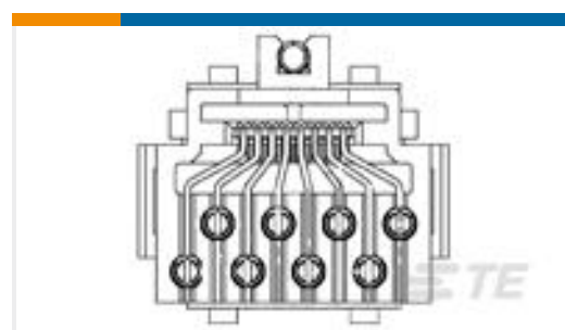
TE 产品编号216811-1 8P. TOOLLESS MOD J.
