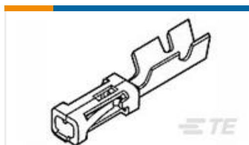
TE 产品编号66360-4 SOCKET ASSEMBLY, LOOSE PIECE, TYPE III+
