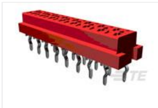
TE 产品编号215079-6 MICRO-MATCH FOB.06P
