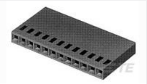
TE 产品编号87499-5 03 MODIV HSG SR MRKD .100CL
