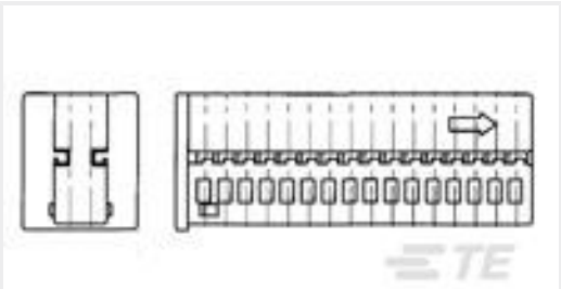
TE 产品编号968265-1 32POS MQS REC
