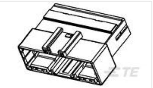
TE 产品编号936211-1 090III 16P CAP ASSY
