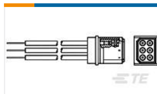
TE 产品编号868021-1 6 POS PLUG ASY W/FLY LEADS
