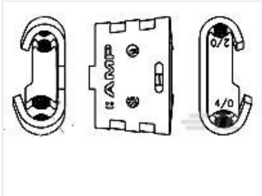
TE 产品编号83631-3 MINIWEDGE,200AMP,4/0-2/0
