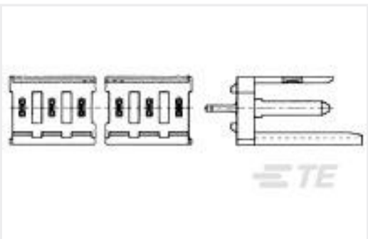
TE 产品编号280614-2 12P MOD 1 SHROUDED HEADER, ST, 0.4 Au
