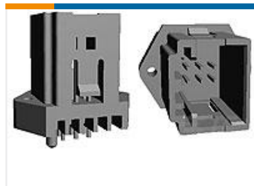
TE 产品编号953363-3 6pos MQS .63 header 180deg
