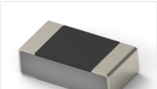
TE 产品编号2176467-3 TLRP 1206 1.0W R012 1% 50PPM 5K RL
