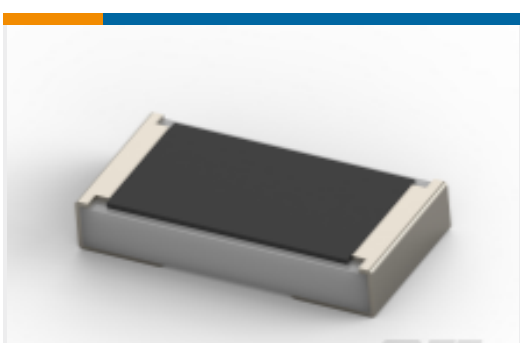
TE 产品编号2176468-1 TLRP 2010 1.0W R010 1% 75PPM 4K RL
