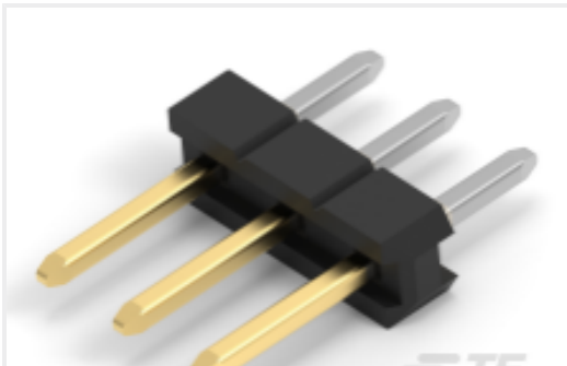
TE 产品编号2355045-3 3P,2MM,BRK HDR,SRVT,2.8,0.1AU,TB
