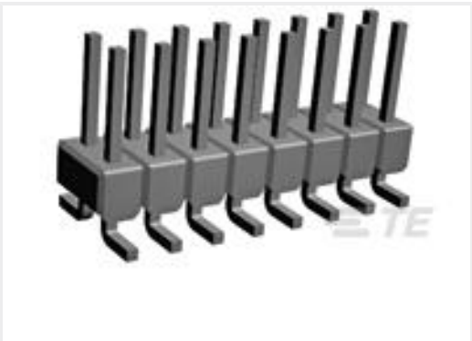
TE 产品编号1241050-8 2x8P MOD II BREAK AWAY HDR,SMD, BLISTER
