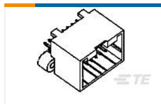
TE 产品编号174973-2 040 MLC CAP ASSY V 12P
