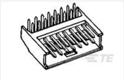
TE 产品编号280389-2 2X4P MODU II SHRD HDR,RT ANG, 0.38AU
