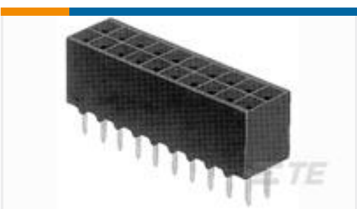
TE 产品编号 2-829410-7 2X27P HV100 REC CON. TE, 6.2MM, TIN
