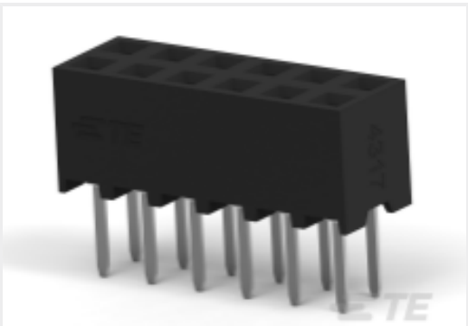
TE 产品编号1-2314820-4 14P,2MM,B-B,REC,DRV,T,2.7,0.1AU,TB
