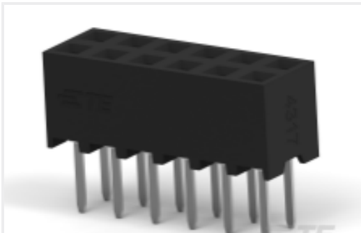
TE 产品编号1-2314820-4 14P,2MM,B-B,REC,DRVT,2,7,0.1AU,TB
