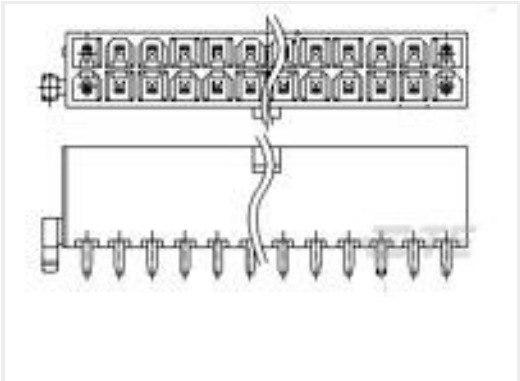
TE 产品编号1-1775099-2 ATX PWR CONN 1 BDLK 4 POS
