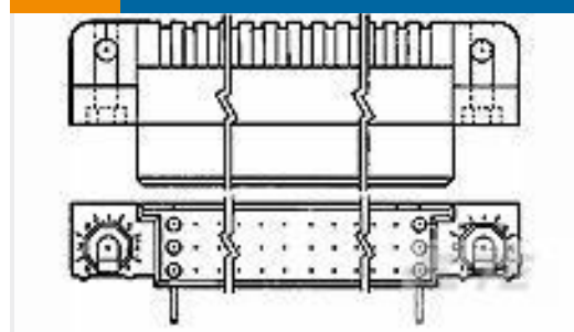
TE 产品编号532834-1 HDI RECP ASSY 3 ROW 165/107
