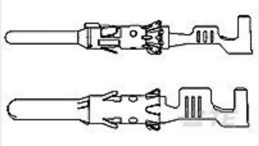
TE 产品编号1703013-1 DIA 1.5MM CONTACT PIN, ASSY
