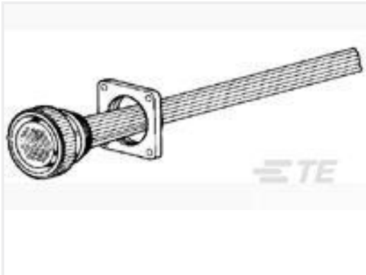
TE 产品编号207299-3 FLANGE PLUG MOUNT CPC
