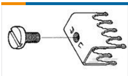
TE 产品编号55323-5 06 PWR TAP CONT PLTD STD .125
