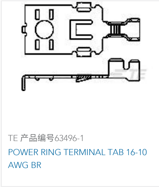
TE 产品编号63496-1 POWER RING TERMINAL TAB 16-10 AWG BR
