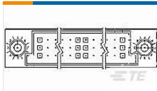
TE 产品编号5532447-5 ASSY,PIN,VERTICAL,HDI,LEAD-FRE
