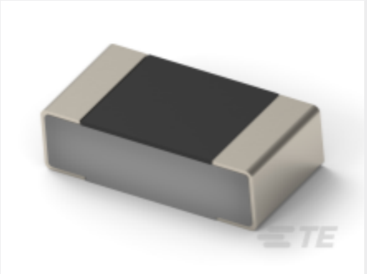
TE 产品编号2176467-6 TLRP 1206 1.0W R025 1% 50PPM 5K RL
