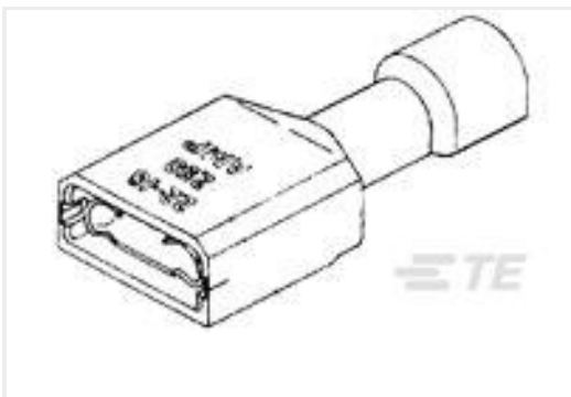
TE 产品编号7-520366-2 ULTRAFAST 110 ASSY REC 26-22 TPBR LP
