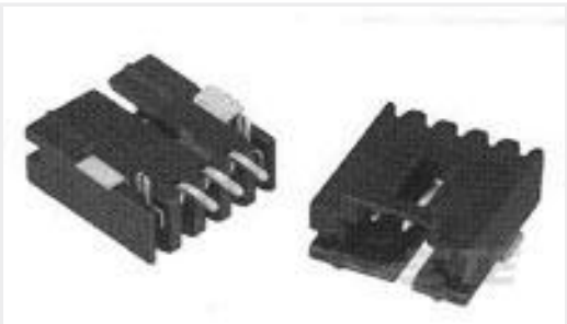
TE 产品编号5-147278-5 06 MTE HDR SRRA SFMNT .100CL
