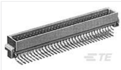
TE 产品编号650946-5 032 EURO TYPE C PIN ST ASSY
